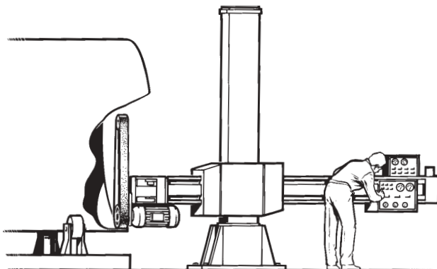
Convert your Welding Boom to a TANK GRINDER
