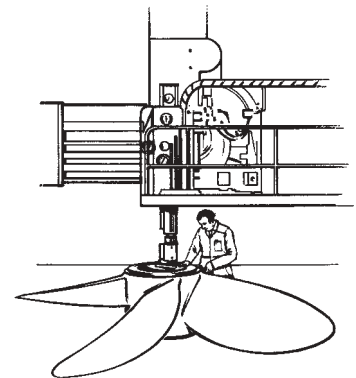
Convert your Vertical Borer to an INTERNAL GRINDER
