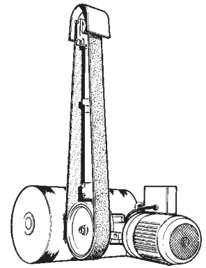
Convert your Lathe to a ROLL GRINDER
