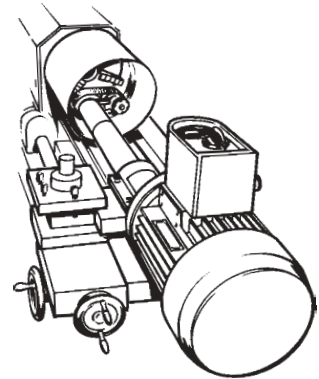
Convert your Lathe to an INTERNAL GRINDER
