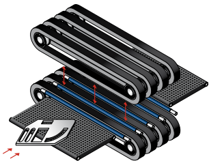
[ XL ] 4/4-AGGREGAT / 4/4-ASSEMBLY
