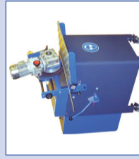
Pedestal chamfering machine. With milling cutters. Max bevel 20mm.
