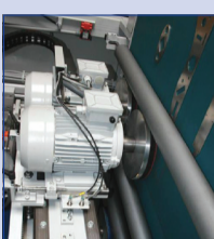
Showing the two disc heads running across the conveyor direction.
